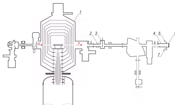
FIG. 1. The layout of the experimental facility: 1 – vacuum insulated tandem accelerator, 2 – non-destructive DC current transformer, 3 – collimator, 4 – target assembly, 5 – \alpha -spectrometer at 135^\circ , 6 – target, 7 – \alpha -spectrometer at 168^\circ
