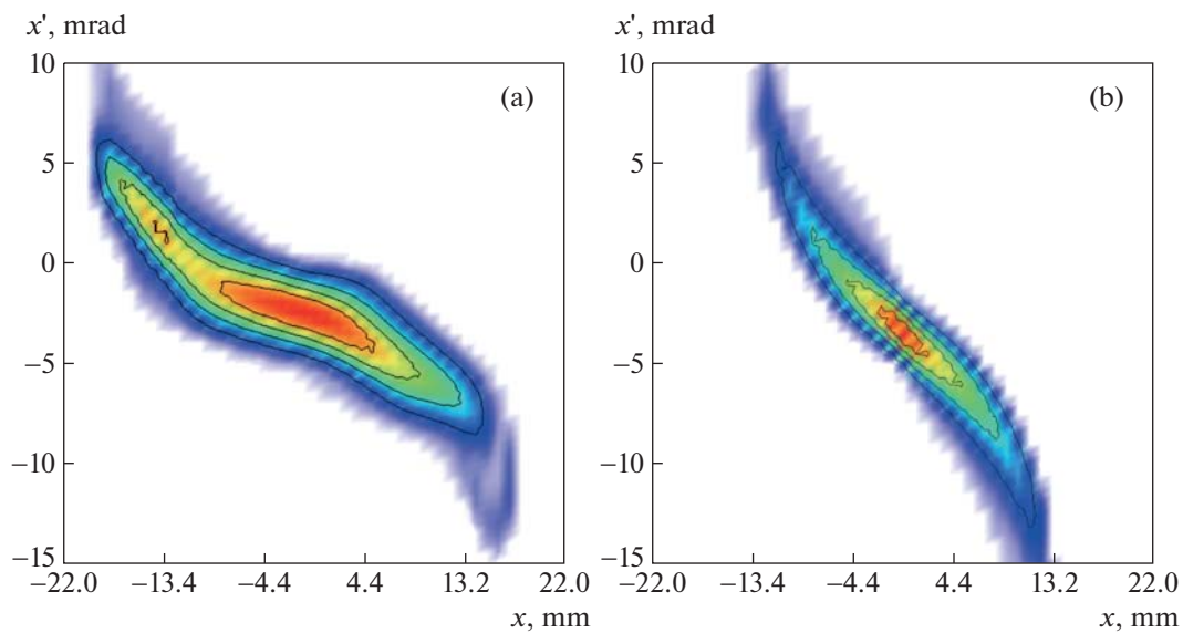
Fig. 5. Phase portrait of a beam of negative hydrogen ions injected into the accelerator with a current of (a) 5 mA and (b) 9 mA.
