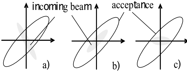
Fig. 7.12. Matching conditions in phase space: mismatch (a), perfect match (b), and efficient match (c)
