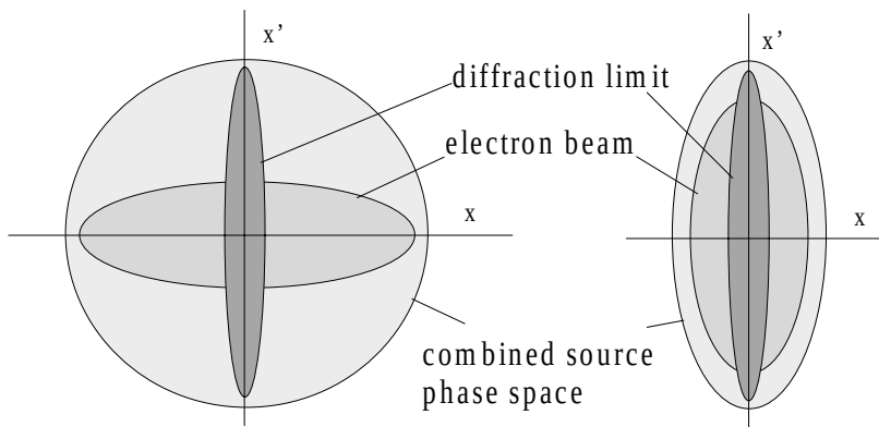
Fig. 21.20. Matching of the electron beam emittance to the diffraction-limited emittance to gain maximum photon beam brightness
