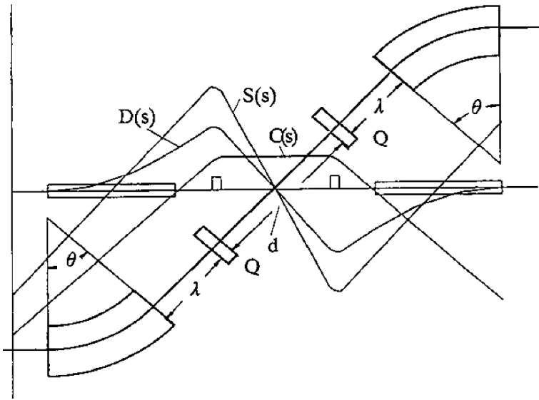
Fig. 5.11. Achromatic beam translation
