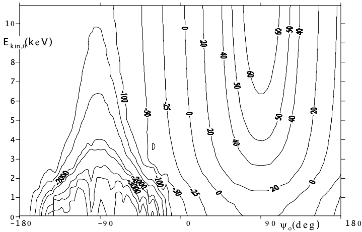
Fig. 15.12. Capture of electrons in a 3 m linac section for initial phase \psi_0 and initial kinetic energy E_{\text{kin},0} . Contour lines are lines of constant particle energy at the end of the section. The phase \psi_0 = 0 corresponds to the crest of the accelerating wave.
