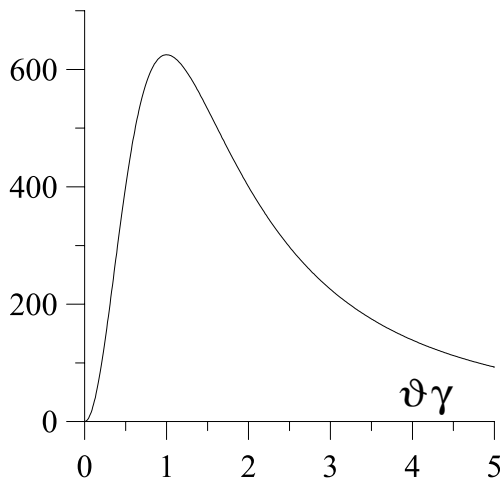
Fig. 22.2. Intensity distribution \frac{d^2\varepsilon}{d\omega d\Omega} \frac{\pi^2 c}{r_c mc^2} of transition radiation
