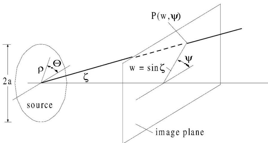
Fig. 21.15. Diffraction geometry
