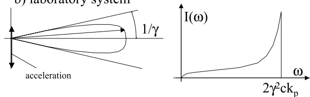
Fig. 21.6. Beam dynamics and spectra radiation lobes, in the particle rest system (a) and the laboratory system (b) for a weak undulator ( K \ll 1 )
