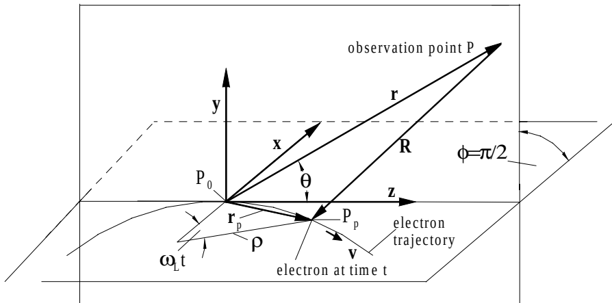
Fig. 22.7. Radiation geometry
