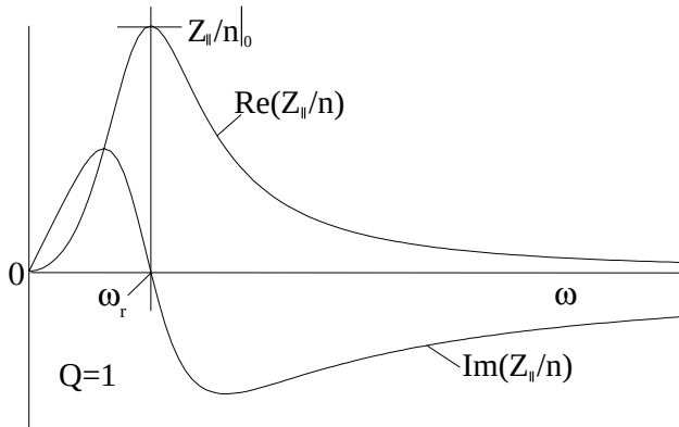
Fig. 19.6. Resistive and reactive broad-band impedance spectrum
