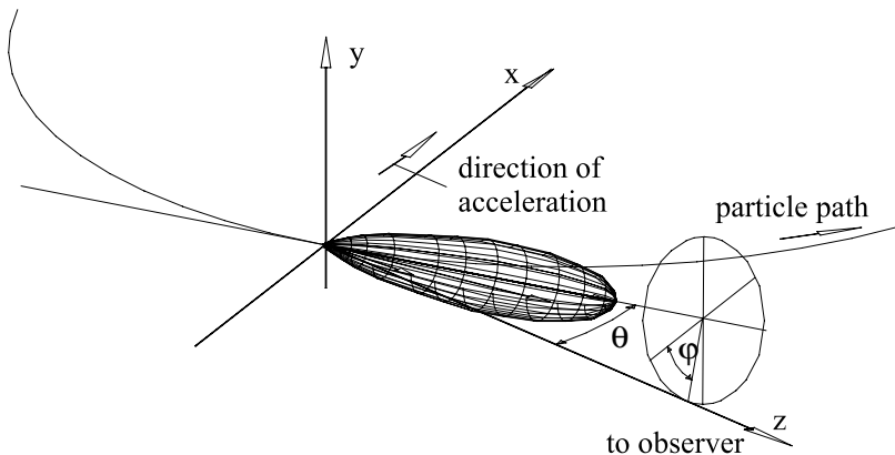
Fig. 22.4. Radiation geometry in the laboratory frame of reference for highly relativistic particles
