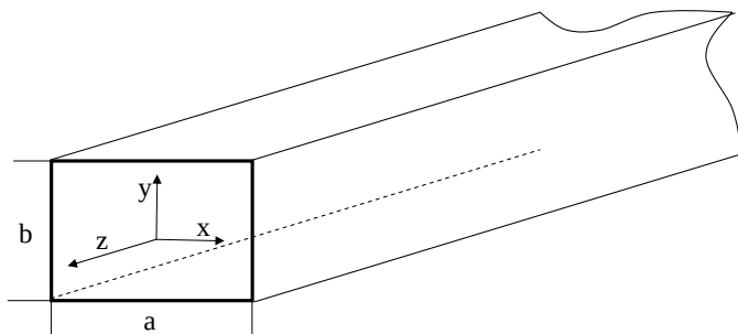
Fig. 15.3. Rectangular waveguide
