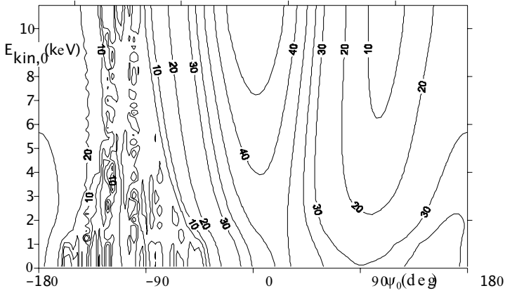
Fig. 15.11. Capture of electrons in a 3 m linac section for initial phase \psi_0 and initial kinetic energy E_{\text{kin},0} . Contour lines are lines of constant particle energy in keV at the end of the section. The phase \psi_0 = 0 corresponds to the crest of the accelerating wave.
