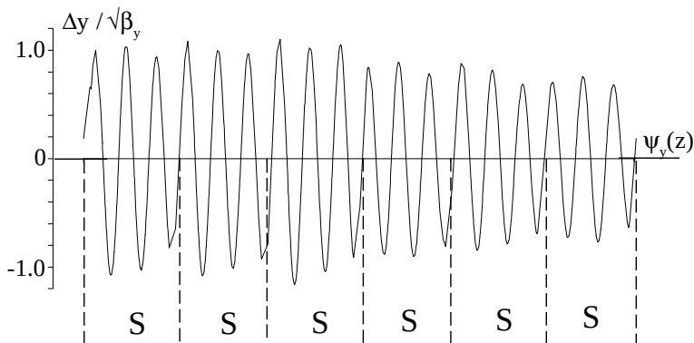
Fig. 12.2. Closed orbit distortion of Fig. 12.2 in normalized coordinates as a function of the betatron phase \psi
