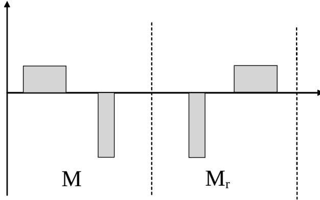
Fig. 4.3. Reversed lattice
