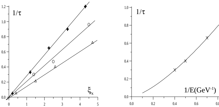
Fig. 19.16. Measurement of the head–tail damping rate in SPEAR as a function of chromaticity (a) and beam energy (b) [227]
